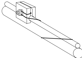
Figure 6 - Lashing Wire Clamp
