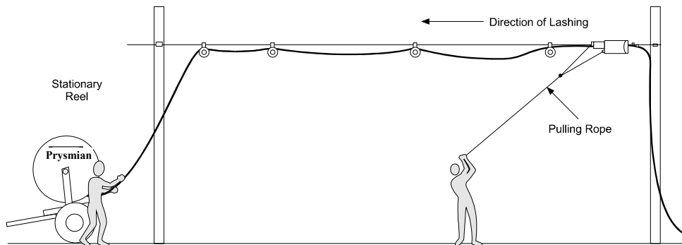
Figure 10 - Pull-back Lashing of Cable
