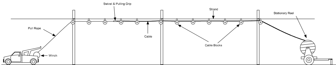
Figure 2. - The Stationary Reel Method of Cable Placement
