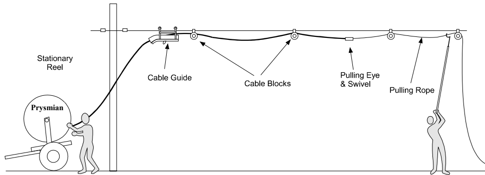
Figure 8 - Setup for Stationary Reel Method
