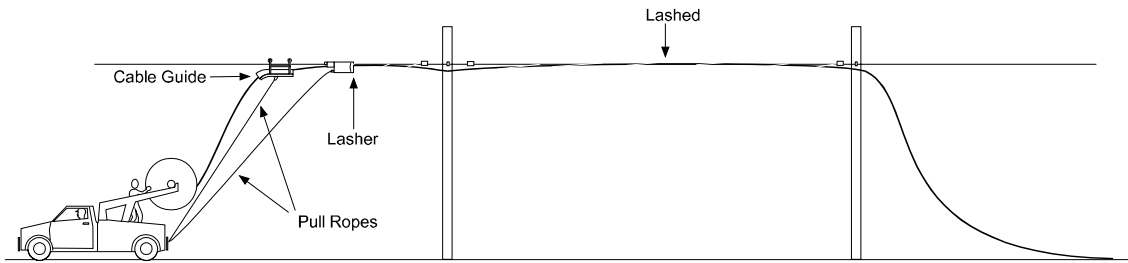
Figure 1. - The Moving Reel Method of Cable Placement
