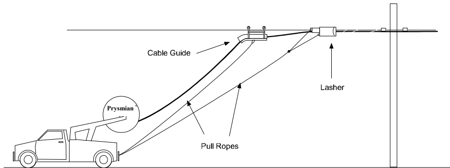
Figure 7 - Setup for Moving Reel Method
