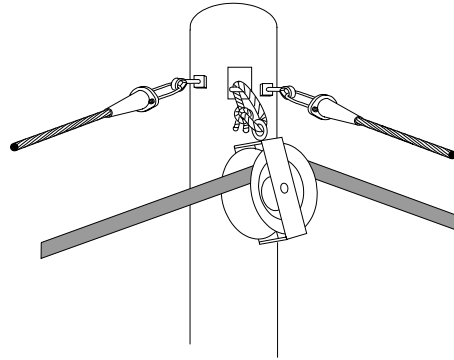
Figure 9 - Snatch Block
