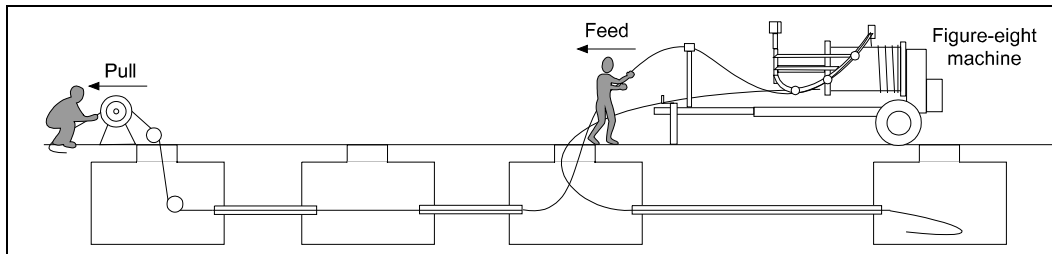
Figure 9 - Pulling Using A Figure-eight Machine
