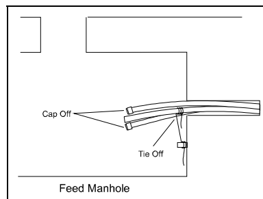
Figure 2 - Cable Tie-off in Manhole
